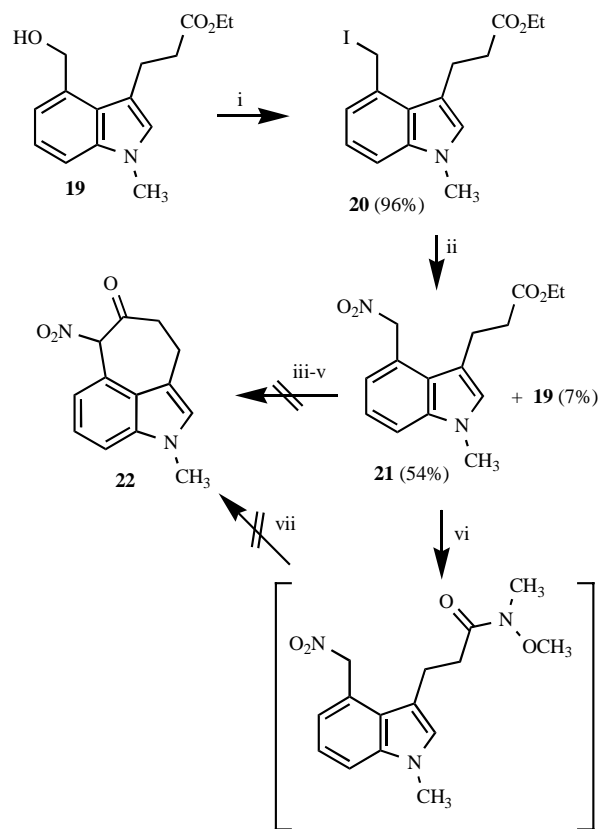
Fig. (5). Installation of a three-carbon chain at the indole C-3 position using diazoalkane and phosphorous ylide chemistry.
