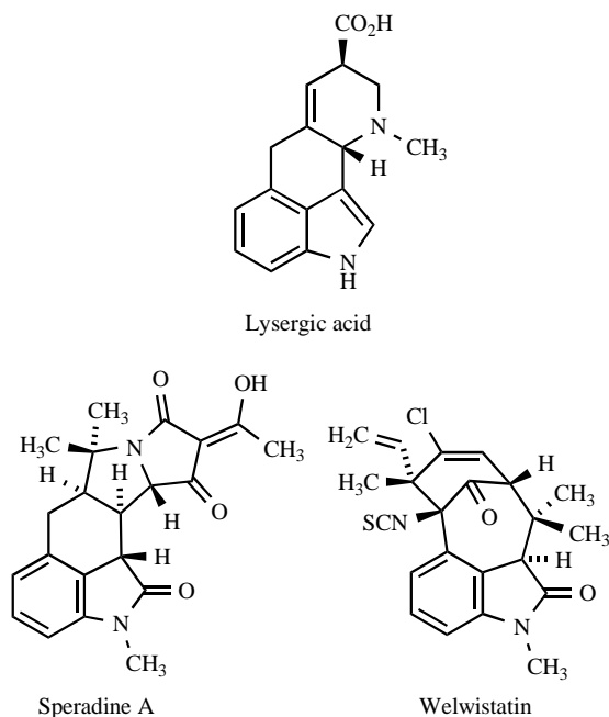
Fig. (1). Structures of some bioactive alkaloids containing a 3,4-disubstituted indole or oxindole fragment.
